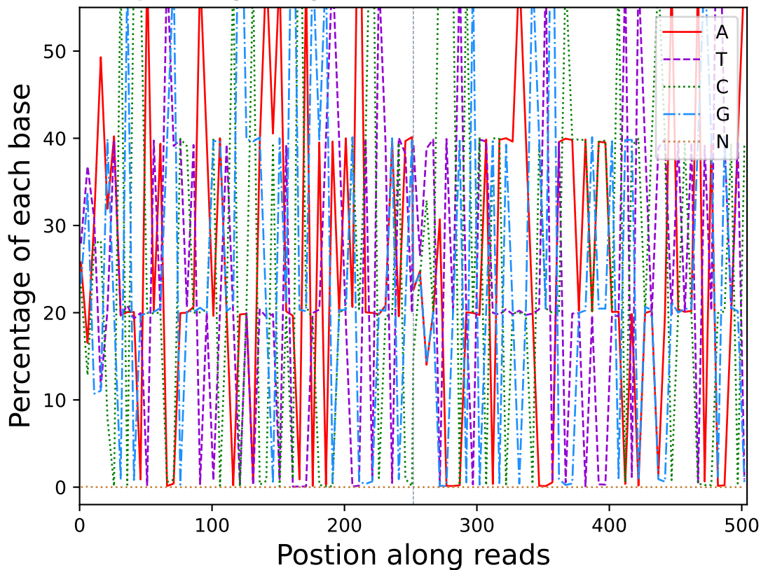
Base percentage along reads (R10902)
